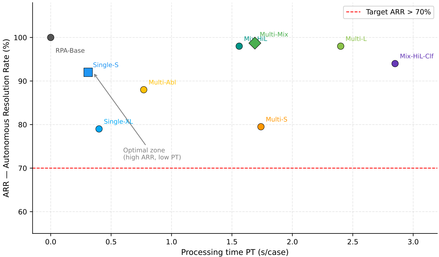
Efficiency frontier: ARR vs. processing time per variant
